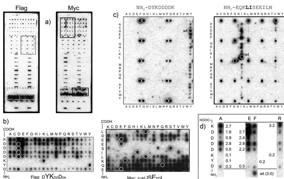
Figure 3. Combinatorial synthesis of a peptide array. Permuted Flag and Myc epitopes were detected by the consecutive addition of epitope-specific mouse monoclonal antibodies (enhanced chemoluminescence luminescence (ECL, Pierce) readout). a) Glass slides with approximately 5500 peptides generated by combinatorial synthesis; the resulting slides were stained with Flag or Myc antibodies. Regularly interspersed positive controls (encircled spots in (b,c)) correspond to wild-type epitopes) and some reactive peptide variants are clearly visible. Frames delineate the enlargements shown in (b,c). b) Characterization of Flag and Myc epitopes. Every amino acid position of each epitope was exchanged for all 20 different amino acids to characterize the binding requirements of epitope-specific antibodies. The epitope specificity deduced from individual experiments is given in the sequence written underneath, whereby the size of an amino acid symbol reflects the importance of that amino acid for antibody binding. The epitope specificities of 9E10 and Flag M2 antibodies agree with published results. [13] c) Epitopes were permuted at the two positions highlighted in bold in the peptide sequence. Interspersed wild-type sequences are encircled. The N-terminal aspartic acid residue of the Flag epitope can be substituted for other amino acids, whereas the adjacent tyrosine residue is mandatory for the binding of the Flag M2 antibody. The highlighted isoleucine residue of the Myc epitope can only be substituted for valine, whereas the adjacent leucine residue is less important for antibody binding. The results of these more complex permutations all agree with the experiments in (b). d) Correlation of the staining intensity of the Flag epitope variants in (b) with published relative affinities, [13] which are written next to the spots stained with the Flag M2 antibody.
