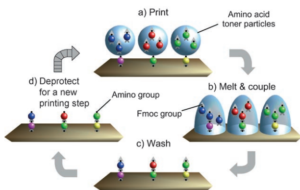
Figure 1. Particle-based Merrifield synthesis. a) A laser printer delivers Fmoc amino acid–OPfp esters embedded within toner particles to specific locations on a solid support, on which b) the particles are melted after transfer. Melting enables the amino acid derivatives to diffuse and undergo coupling to the support. A synthetic cycle is completed when c) excess monomers are washed away, and d) the Fmoc protecting group is removed. Repeated coupling cycles generate a peptide array.
