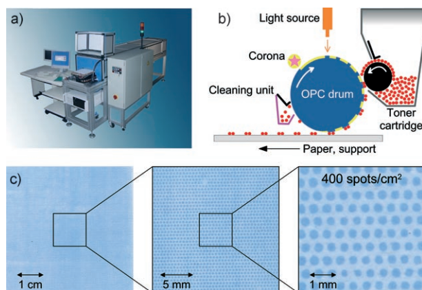
Figure 2. Laser printing: a) The peptide laser printer with 20 different printing units aligned; the mounting for the support is visible at the front of the printer. b) A light source (LED row, orange) illuminates and thereby neutralizes selected areas of an OPC drum (blue), which is first uniformly charged (yellow) by a corona. Triboelectrically charged toner particles are transferred to these neutralized areas and from there by a strong electric field to a solid support. c) Amino acid toner was printed by the peptide laser printer onto a glass slide derivatized with free amino groups. The esters (in this case: Fmoc-Ile-OPfp) embedded in the particles were released by heat, the residual material was washed away with DMF, and the remaining free amino groups were blocked with 10% acetic anhydride in DMF. Finally, the Fmoc protecting groups were removed with 20% piperidine in DMF, and the newly introduced free amino groups were stained with 0.1% bromophenol blue in methanol.
